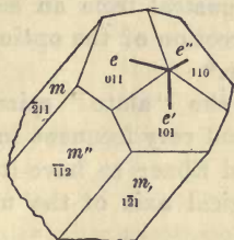
FIG. 8 (from a drawing by Professor Lewis).—Crystal of calcite infiltrated by opaque black matter (probably a metallic oxide), which forms a three-rayed star, shown by the strong short lines in the diagram. The rays bisect the angles made by the edges of the faces e , e' , e'' , and therefore lie in the planes of symmetry of the crystal. The black matter is in part underneath the faces, so that the reflecting surface can be seen to be uninterrupted over it. The specimen in the Cambridge Collection contains upwards of 120 crystals in which the star is conspicuously seen.
